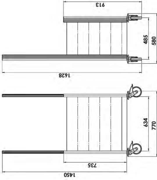
Case for 5 height grids with extended profile supports at rear
