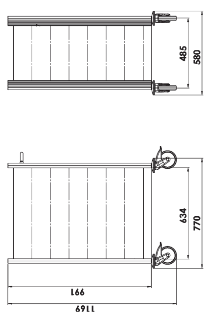
Case for 7 height grids
