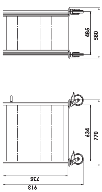
Case for 5 height grids
