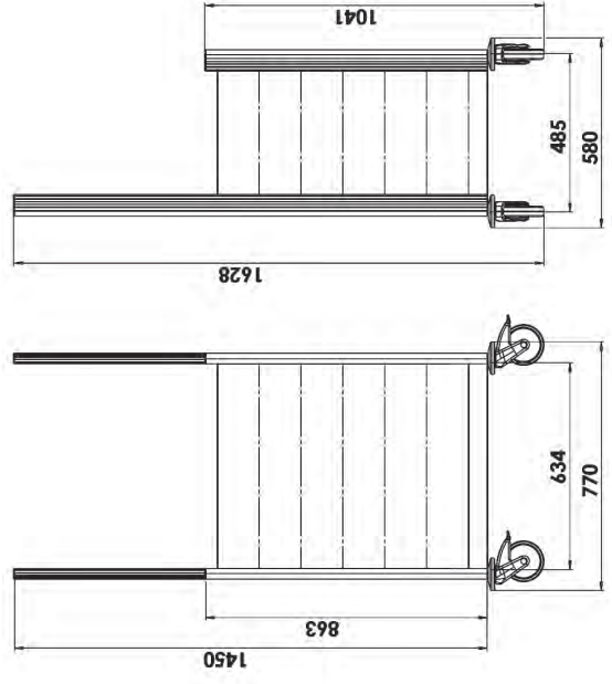
Case for 6 height grids with extended profile supports at rear
