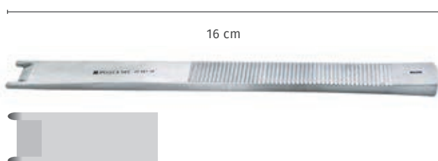
Masing Osteotom, 2 Führungsdorne, 10 mm-Schneide, gerade, 16 cm Masing osteotome, 2 guards, 10 mm blade, straight, 16 cm 20-441-16
