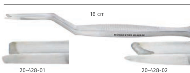
Killian-Claus Hohlmeißel, bajonett, 5,5 mm, 16 cm Killian-Claus gouge, bayonet, 5.5 mm, 16 cm
