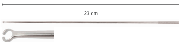
Knotenführer, gerade, AL 23 cm / Knot tier, straight, WL 23 cm
